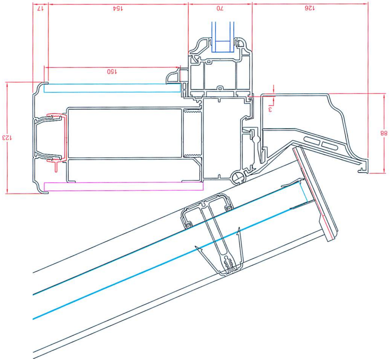
PVC Gutter & Capella Soffit
