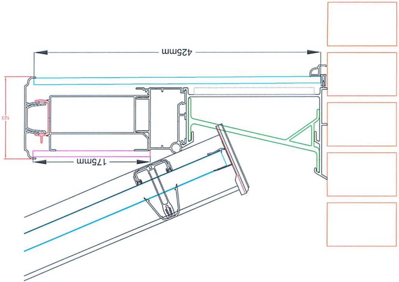
210mm Box Gutter & Capella Soffit
